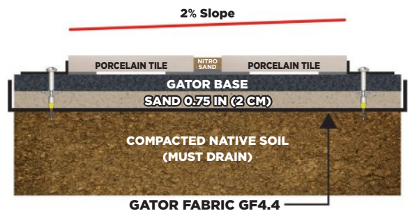
CROSS SECTION OF THE GATOR TILE SYSTEM
